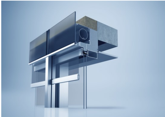
[Photo: heroal VS Z in the facade heroal C 50]
